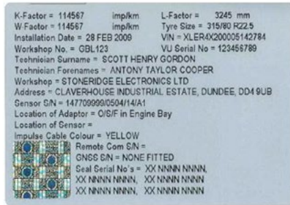
CALIBRATION LABELS FOR THERMAL PRINTER
